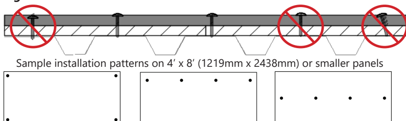
Figure H. ESD Screw Installation - Cross Section - Screws must be flush with deck surface!
